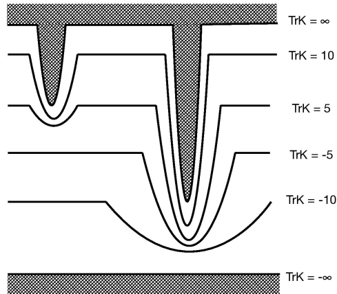
Figure 1: A depiction of York time in a spacetime with singularities. Adapted from similar figures in (Qadir and Wheeler, 1985).
