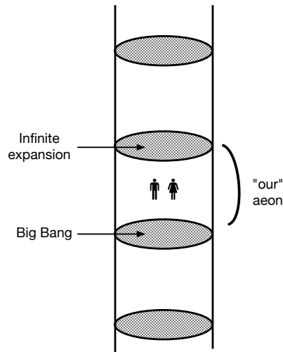
Figure 2: Aeons of time in a conformal cyclic universe.
