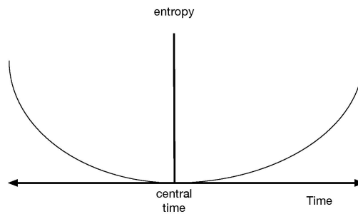
Figure 3: The arrow of time aligning with increasing entropy in “two-sided” universes.
